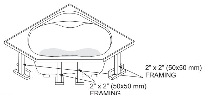
FIGURE 2 SUPPORT CORNER TUB INSTALLED WITH APRON
