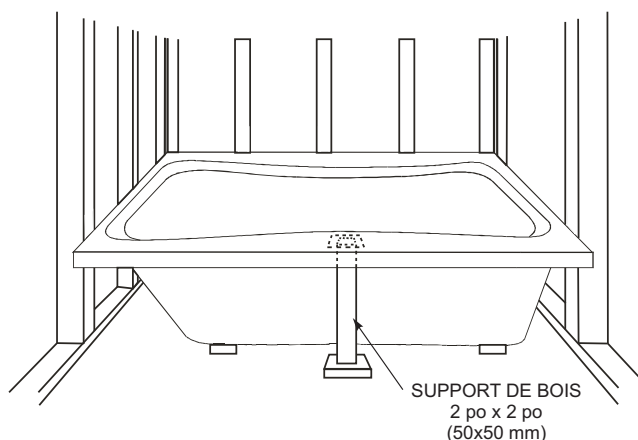
FIGURE 1 - INSTALLATION EN ALCÔVE
