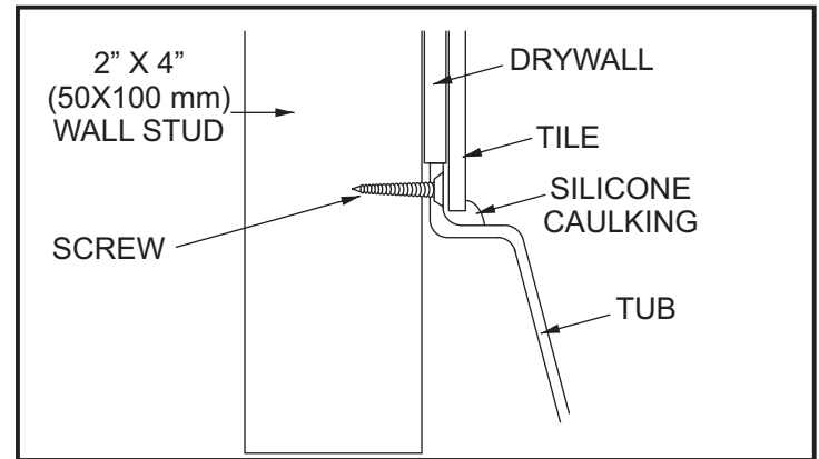
FIGURE 5 - WALL INSTALLATION FOR TUBS WITH TILE FLANGE
