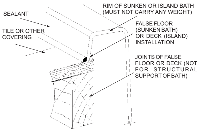
FIGURE 6 - METHOD OF SUPPORTING RIM OF SUNKEN OR ISLAND BATH
